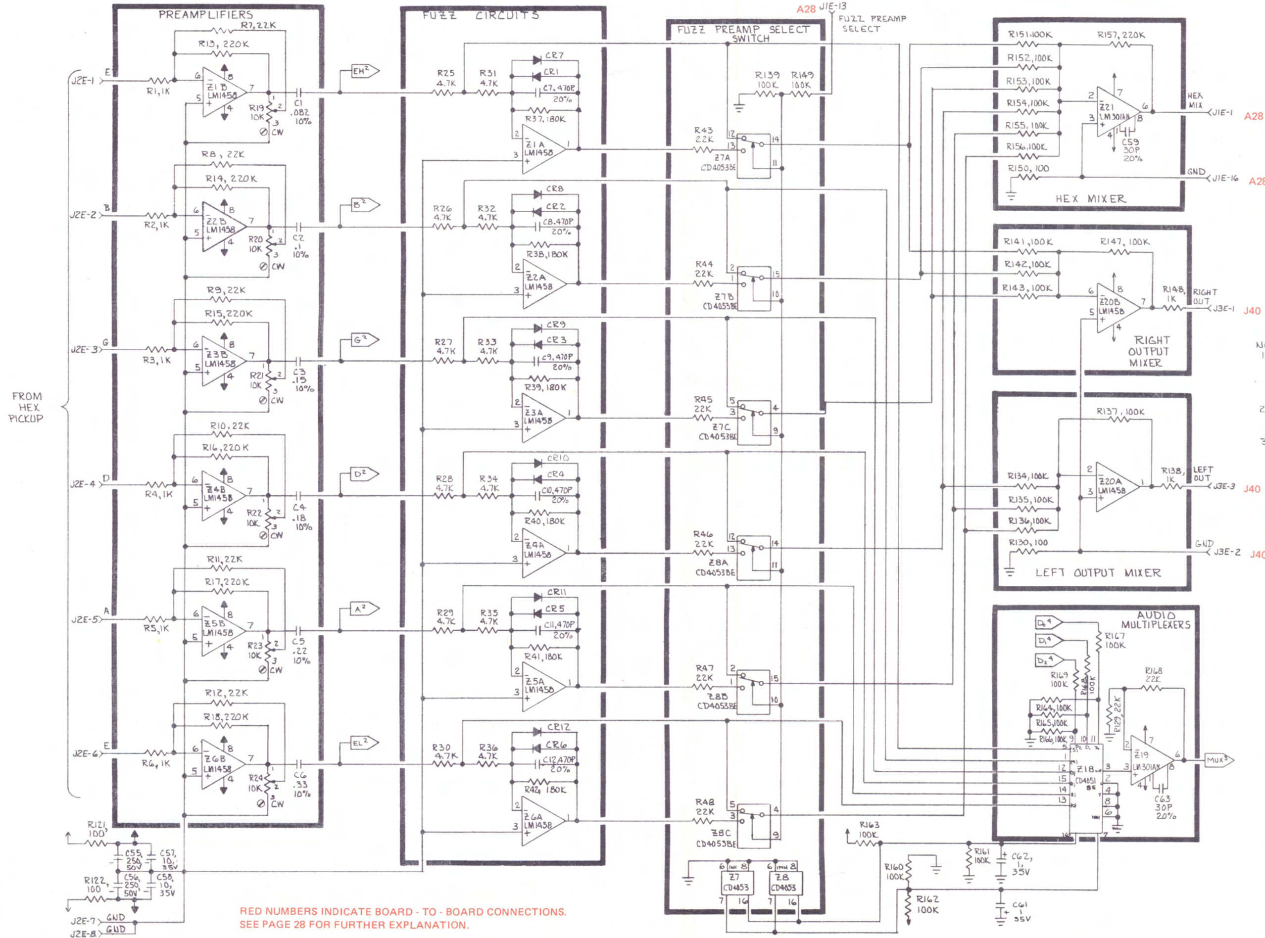
AVATAR MODEL 2223 SCHEMATIC BOARD E 1 OF 3
