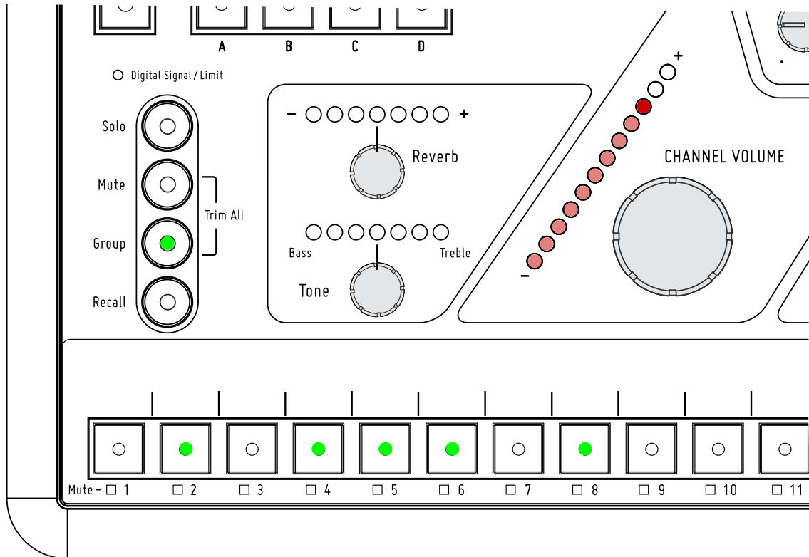
In this example, mix channels 2, 4, 5, 6, and 8 are grouped together. The Channel Volume knob controls the Group volume.
