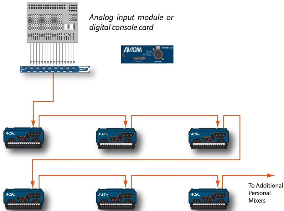
A typical daisy chained Pro16 personal mixing system with six A-1611 mixers is shown.
