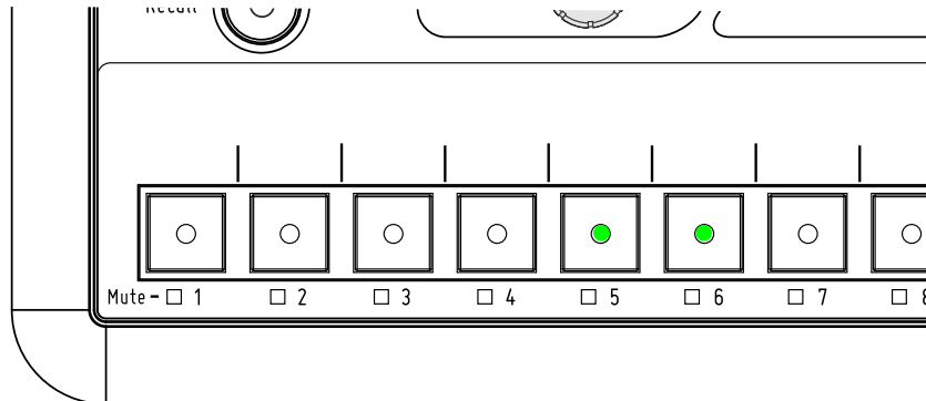
Channel 5-6 are stereo linked at a Pro16 input device; the rear panel mode switch is set to Pro16.
