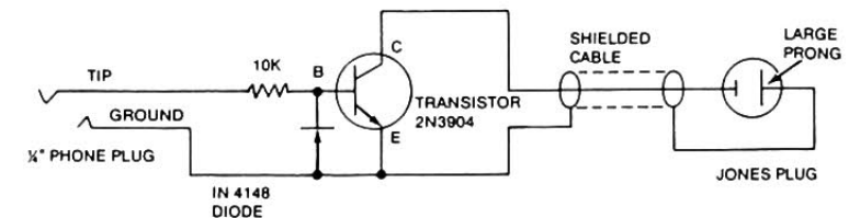
V-TRIG TO S-TRIG CONVERSION CIRCUIT
