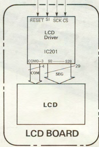
TR-505 BLOCK DIAGRAM
