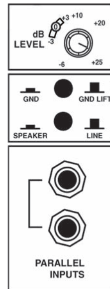
NX200S Rear Panel
